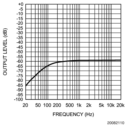
Channel Separation R_L = 16\Omega , P_O = 5mW Single Ended Output, A_V = -1
